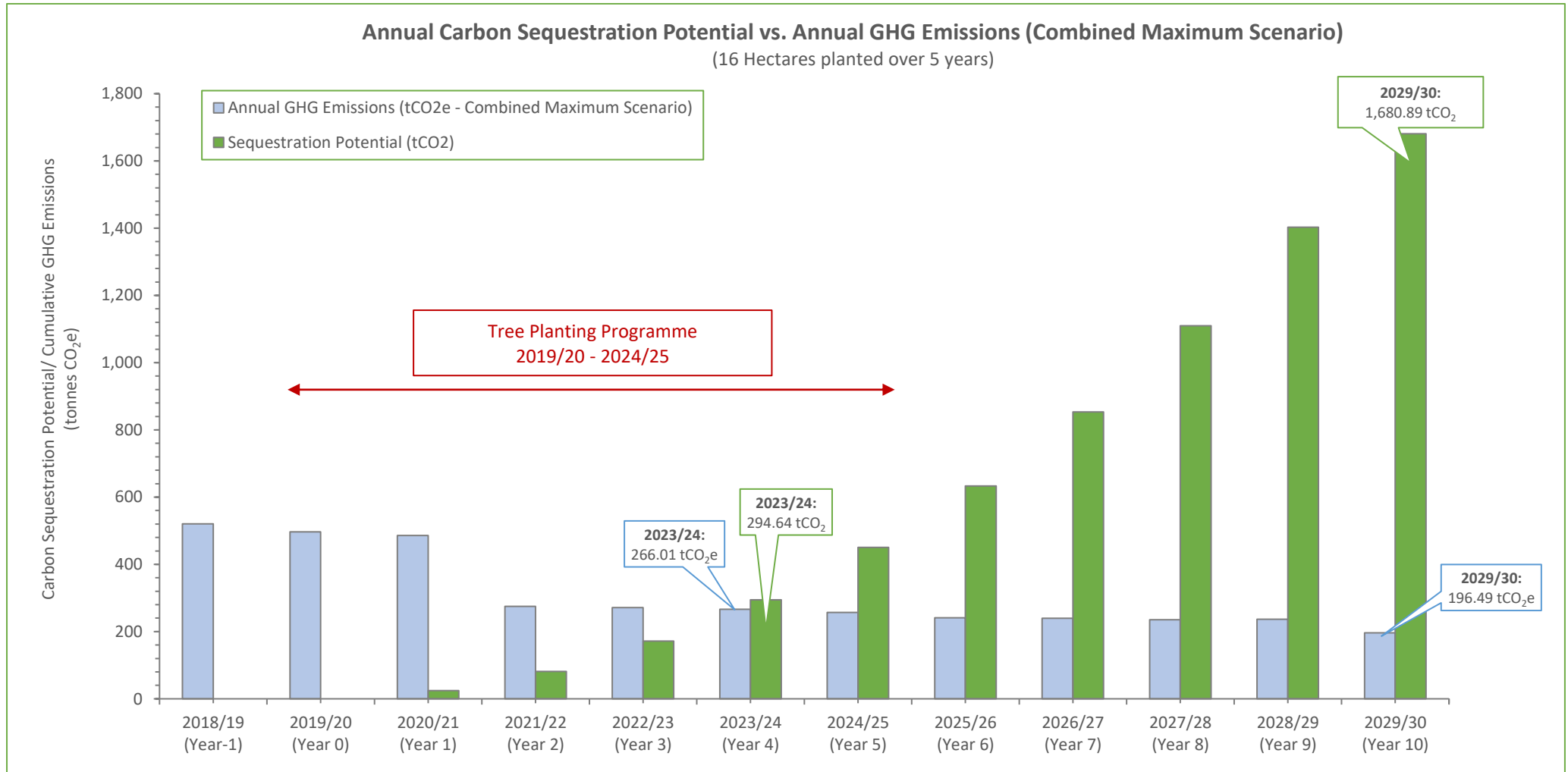
Figure 7 - Carbon sequestration potential of planting 16 hectares of UK native trees over 5 years (based on Combined Maximum scenario) compared with annual GHG emissions.
