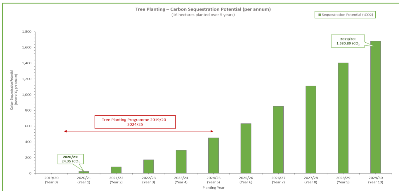
Figure 4 - Carbon sequestration potential (tonnes CO 2 ) for 16 hectares of UK native trees planted over 5 years (c.3.4 ha per annum between 2020/21 and 2024/25)
